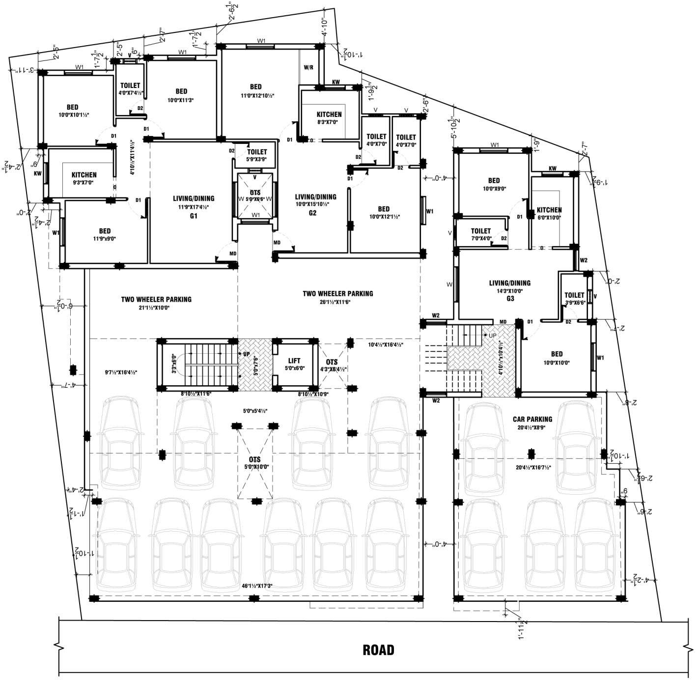
SITE CUM GROUND FLOOR PLAN
